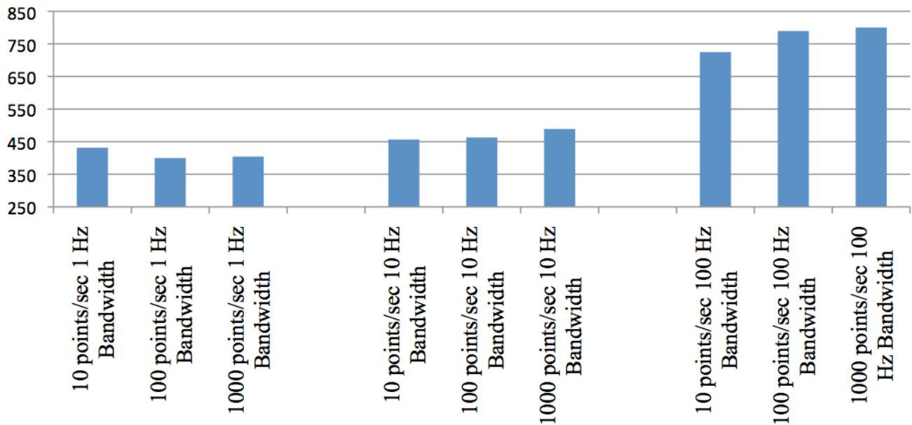
Chart 2. "Mean" Maximum Load (gf)
